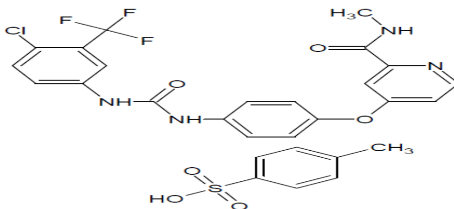
Figure 6: 4-(4-(3-(4-chloro-3-(trifluoromethyl)phenyl)ureido)phenoxy)-N2-methylpyridine-2-carboxamide-4-methylbenzene sulfonate.
